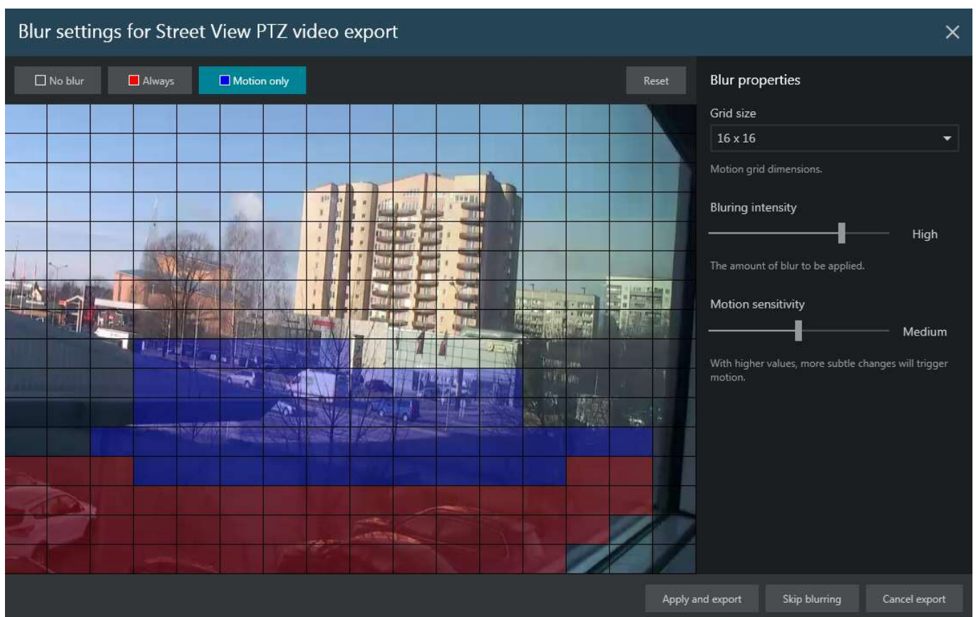
Privacy masking using motion blur
